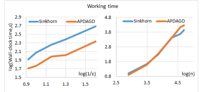
Figure 1. Comparison of working time of Algorithm 2 (Sinkhorn's algorithm) and Algorithm 4 (APDAGD).
